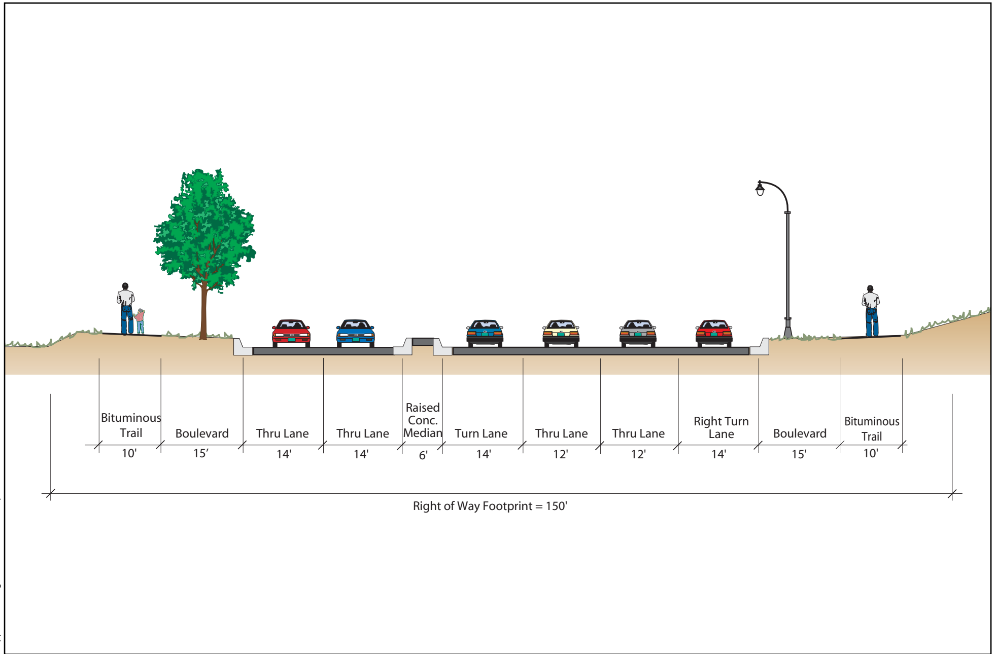
FOUR-LANE URBAN SECTION - CSAH (Turnlanes at intersections) NORTHEAST WRIGHT COUNTY SUB-AREA STUDY
