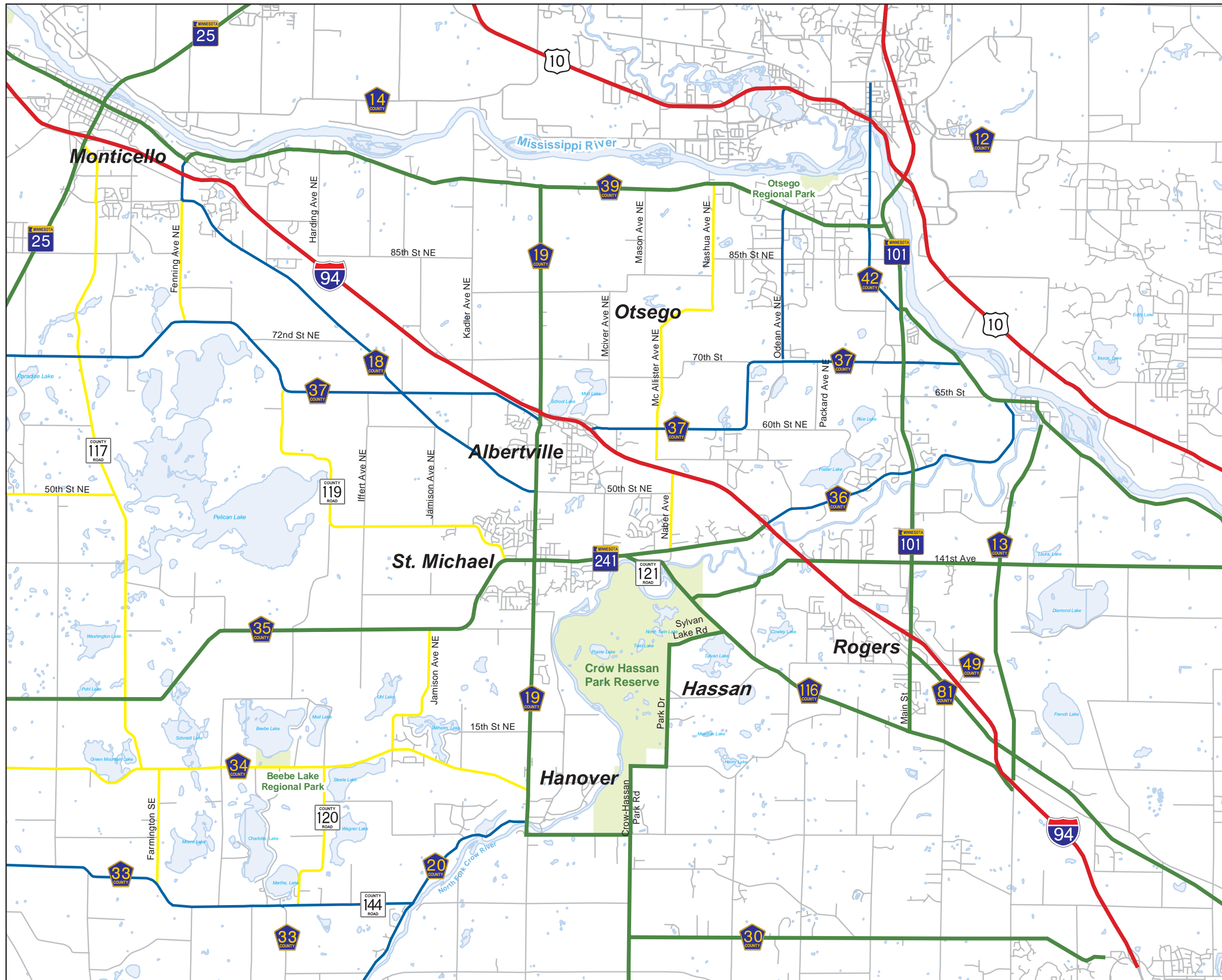
Figure 7 Existing Roadway Functional Classification
